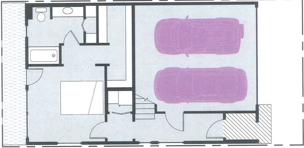
FIRST FLOOR 460 SQ. FT.
